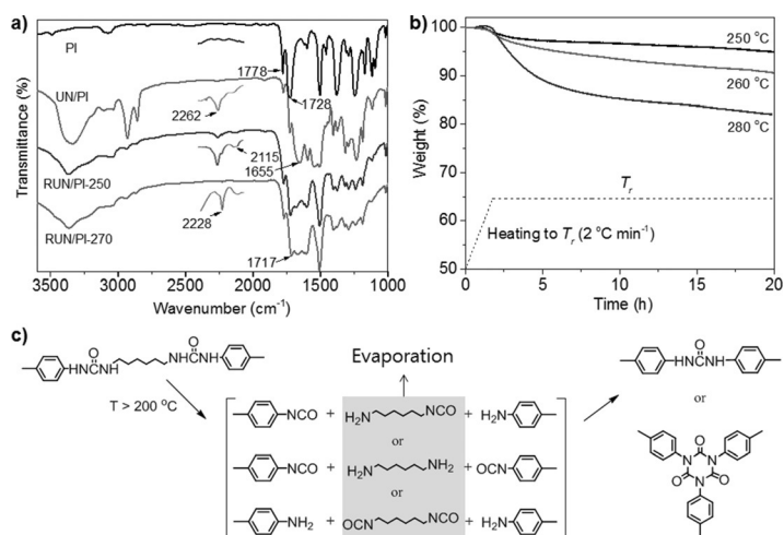
Figure 3. Rearrangement of UN to RUN in the nanocomposite blends. a) FT-IR spectra of the PI, UN/PI, and RUN/PI ( W_p=0.1 ). The “RUN/PI-250” and “RUN/PI-270” labels refer to the RUN/PI films treated at T_r=250 and 270 °C, respectively. b) TGA data obtained at isothermal conditions at 250, 260, and 280 °C, respectively, using UN/PI ( W_p=0.4 ). Note that FT-IR spectra were obtained from the blend with a low PI content to better show the structural change of UN. c) Scheme of the thermal rearrangement of urea bonds.
